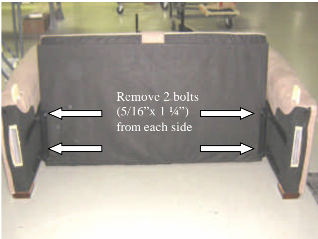
7. If more height reduction is required then remove the back bed section
