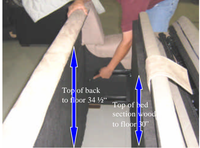
2. Remove one bolt (5/16" x 2 1/4") from each inside arm. Removing back drops the height 4 1/2" Removing legs drops the height 1 1/2" - 2" more
